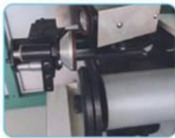
動力修刀裝置 (選裝) Power tool trimmer (optional)
